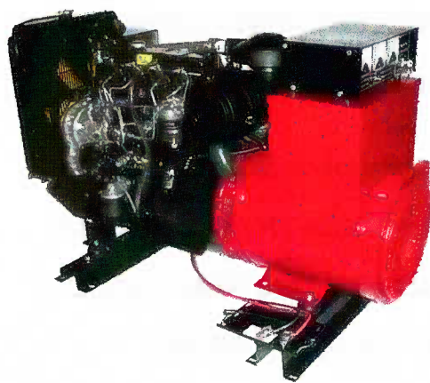
OPEN GENERATOR SET FOR INSTALLATION IN UN-INHABITED BUILDING.
